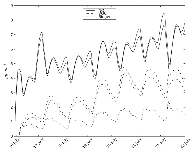
Figure 15. Time evolution of the standard deviation (averaged over the whole domain) of the ensemble for first-layer ozone concentrations. It is shown for NO, VOC and biogenic emissions for the full ensemble (200 simulations) and for a restricted ensemble (100 simulations).
