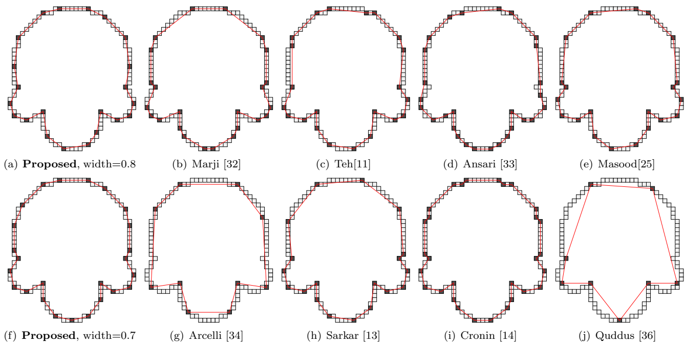
Figure 11: Dominant points of the semicircle curve.
