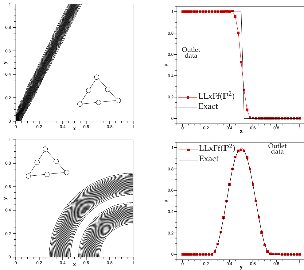
Figure 6: Rotation problem : Results obtained with the scheme (4.4)–(4.9) for \mathbb{P}^2 interpolation. Top : result for problem (6.1) ( \min = -1.0094 , \max = 1.01 ). Bottom : results for problem (6.2) ( \min = -0.1735 \cdot 10^{-4} ). The first order scheme is (4.8).
