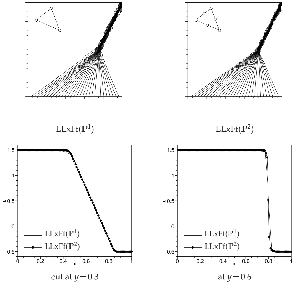
Figure 7: Burger equation, solution obtained with a P^1 and P^2 Lagrange interpolated and the scheme (4.4)-(4.9).
