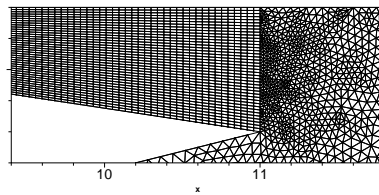
Figure 12: Zoom of the mesh for the Scramjet problem.
