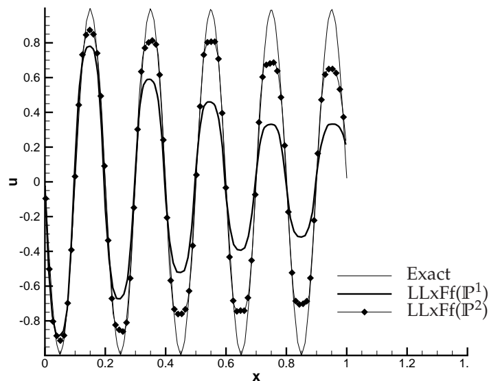
Figure 3: Rotation of the smooth profile: u_{in} = \sin(10\pi x) . Computed outlet profile. All computations run on the same number of degrees of freedom. Reference mesh size h=1/80 .
