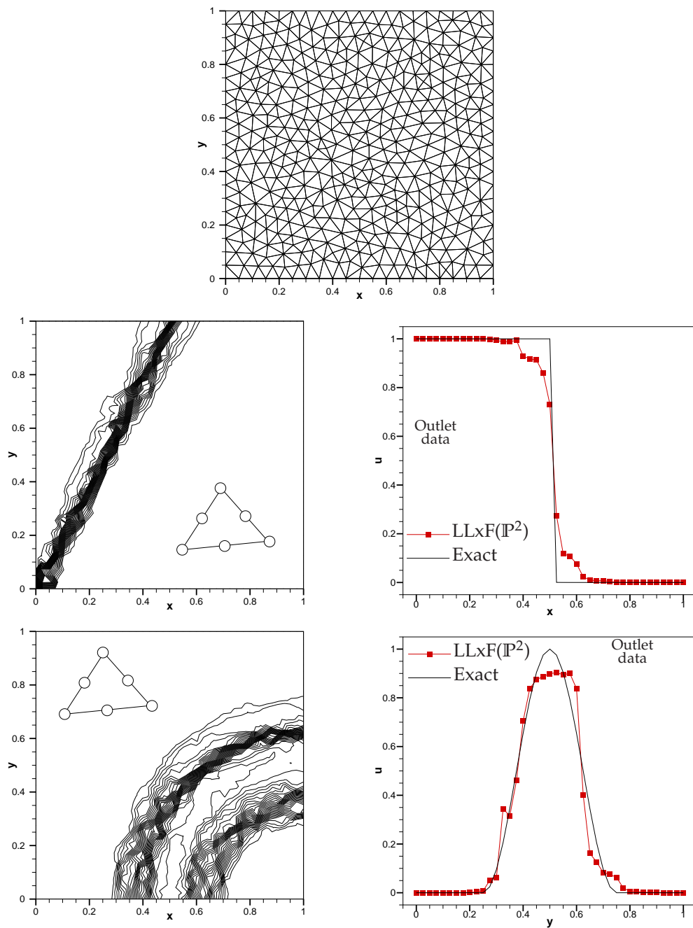
Figure 4: Convection problem : Results obtained with scheme (4.3)–(4.9) for \mathbb{P}^2 interpolation. Top : mesh. Middle : result for problem (6.1). Bottom : results for problem (6.2). The first order scheme is (4.8).
