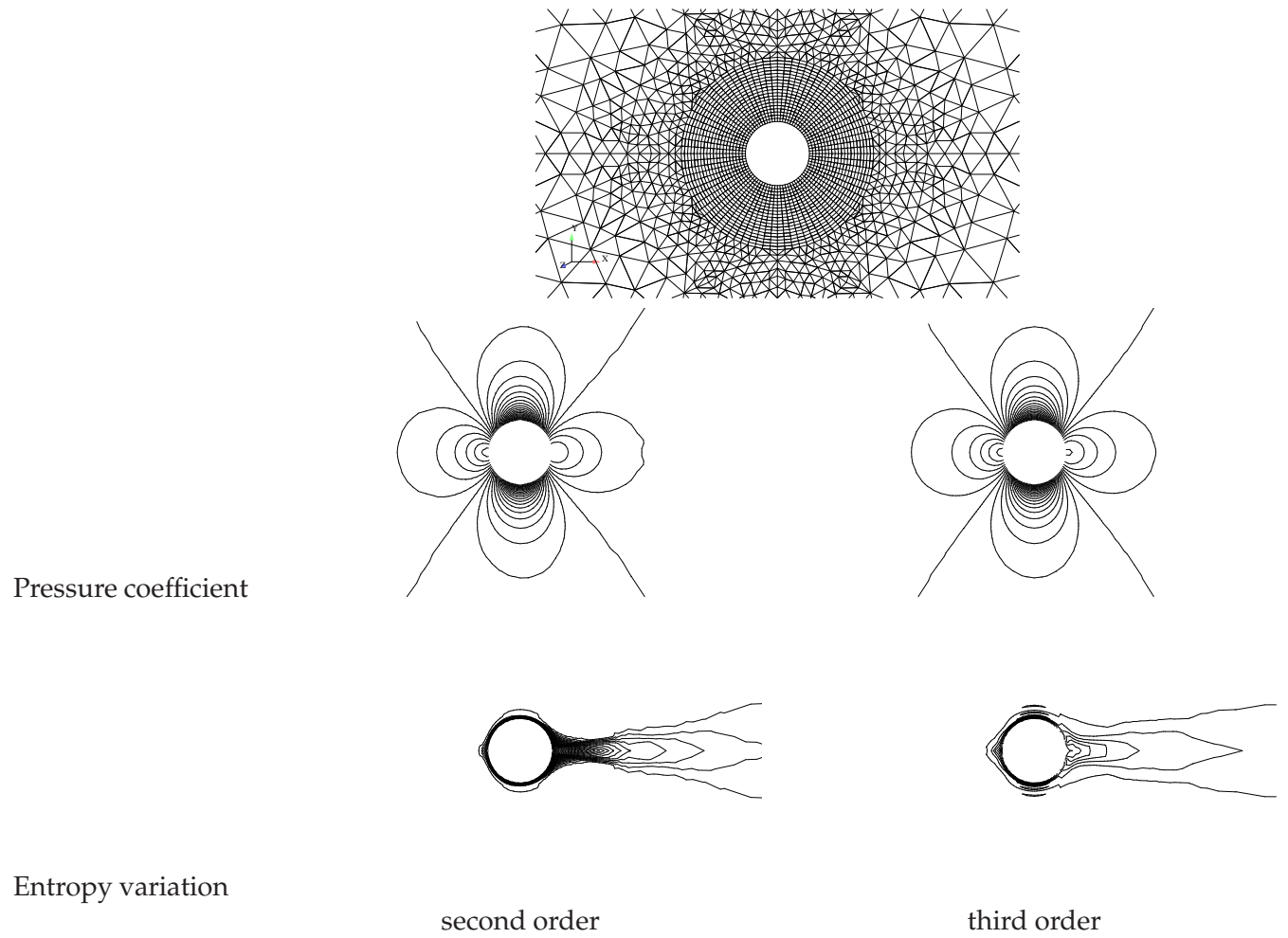
Figure 11: Subsonic sphere problem, hybrid mesh : Pressure coefficient and entropy variation on an hybrid mesh, M_\infty = 0.35 .
