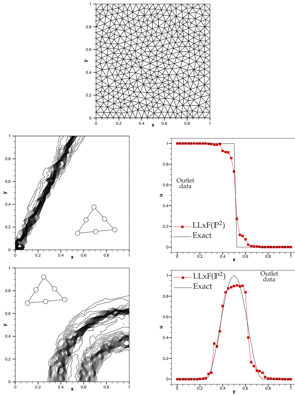
Figure 4: Convection problem : Results obtained with scheme (4.3)–(4.9) for P^2 interpolation. Top : mesh. Middle : result for problem (6.1). Bottom : results for problem (6.2). The first order scheme is (4.8).
