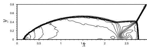
Figure 14: Double Mach reflection. Density contours. 30 equally spaced contours from 1 to 24. Taken from [32].
