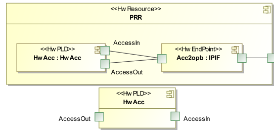
Fig. 8. A Reconfigurable Hardware Accelerator
