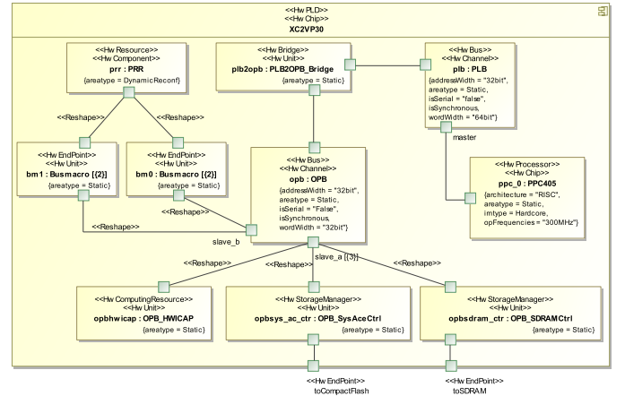
Fig. 9. Modeling of our PDR Architecture
