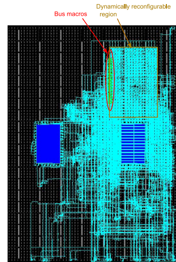
Figure.13: Full bitstream related to the reconfigurable SoC
