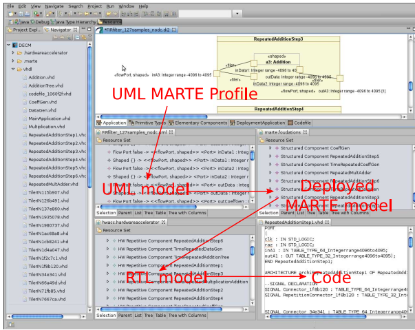
Figure.10: The transformation flow related to our design flow
