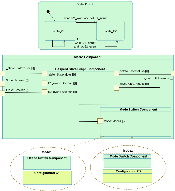
Figure.8: Modeling mode automata concepts at Gaspard2 IP deployment level
