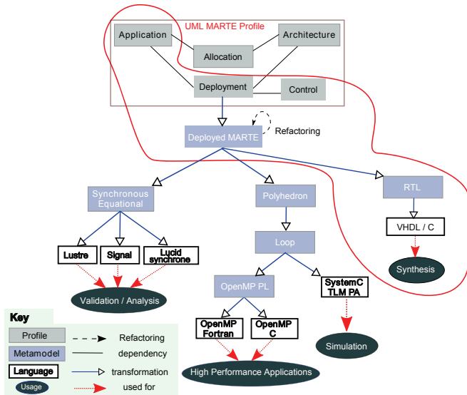
Figure.1: Overall view of Gaspard2 framework with emphasis on our specific contributions
