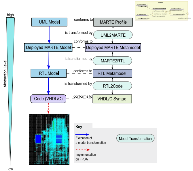
Figure.2: An abstract overview of the model transformation chain. Several intermediate metamodels help to bridge the gap between high level modeled UML diagrams and the final RTL code generation
