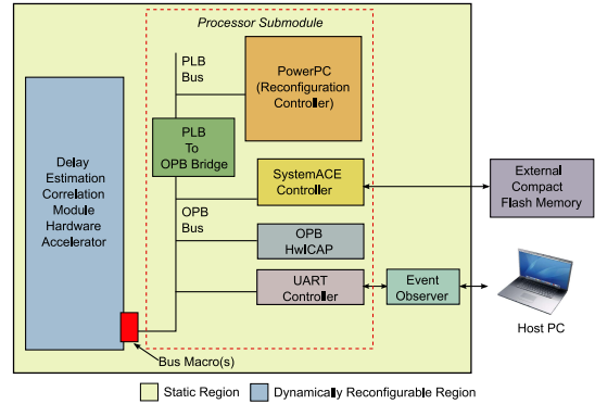
Figure.12: Block Diagram of the architecture of our reconfigurable system
