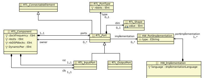
Figure.9: An extract of the RTL metamodel related to component ports and associated types
