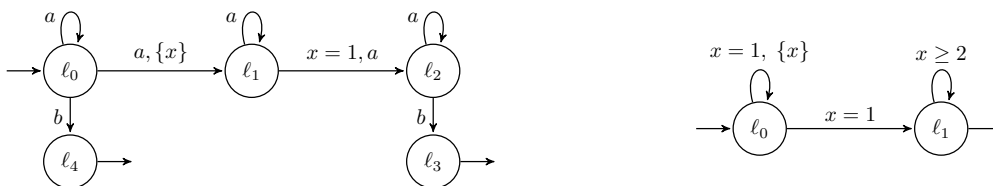
Figure 6: Examples of determinizable TA not treatable by [BBBB09a].
