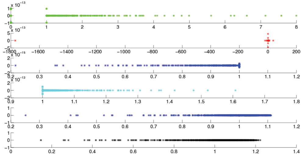
Figure 4: Spectrum plot of from top to bottom : NMLUR, NMLUC, NSSOR, ILUNO, ILUND, and MILU for the matrix 3dCS15, nparts=8. Horizontal axis: real part of eigenvalues, vertical axis: imaginary part of eigenvalues
