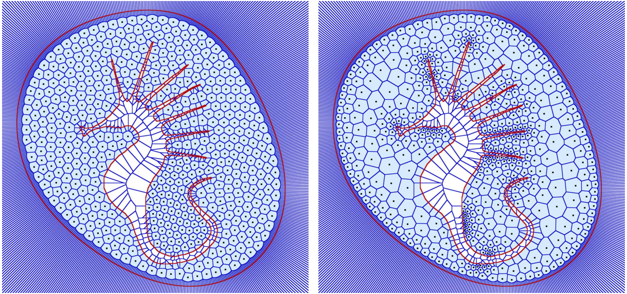
Figure 8: result 2. uniform and adapted k = 0.1
