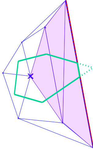
Figure 4: Construction of a cell of the bounded Voronoi diagram. The standard Voronoi diagram is truncated on the constrained edge (colored triangles are blind).
