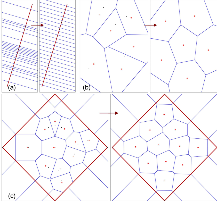
Figure 6: Lloyd iteration with a uniform density. (a) Vertices randomly located on a constrained edge, and after convergence of the Lloyd iteration. (b) Vertices randomly located in a 2D domain, and after convergence of the Lloyd iteration. Sites are filled dots, and centroids are outlined dots (they coincide after convergence). (c) Lloyd iterations applied both in 1D and 2D.
