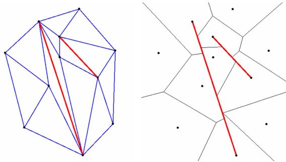
Figure 3: Constrained Delaunay triangulation of a set of points (left) and its pseudo-dual bounded Voronoi diagram (right).
