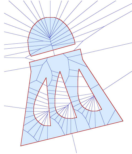
Figure 5: Bounded Voronoi diagram of a PSLG.
