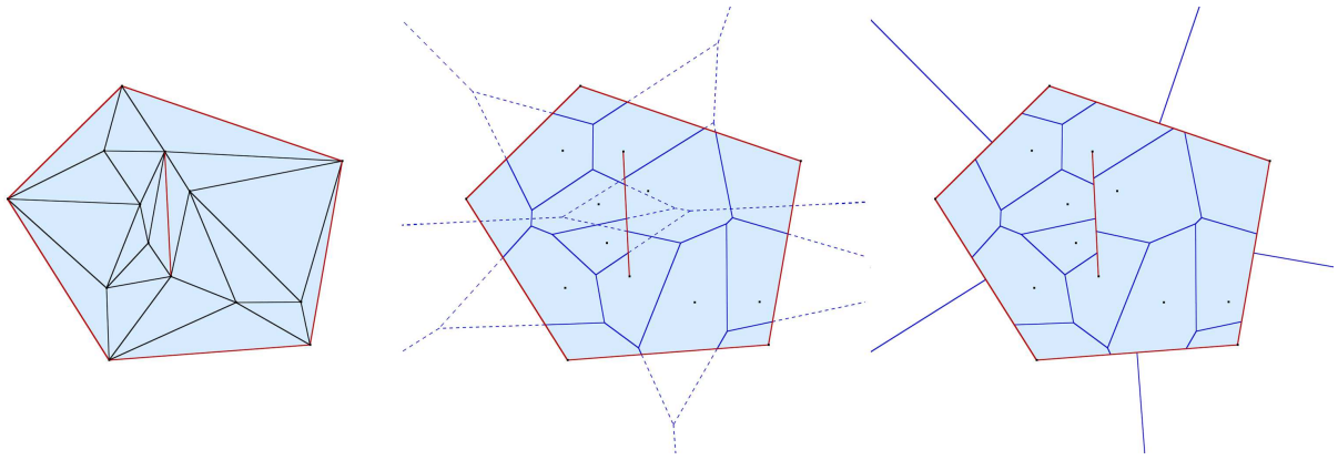
Figure 1: (Left) CDT: Constrained Delaunay triangulation of a set of vertices. (Middle) Constrained Voronoi diagram: CVD, standard dual of the CDT. (Right) BVD: Bounded Voronoi Diagram.
