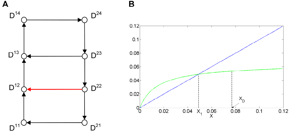
Figure 11. Transition graph and first return map for the modified Model 3. (A) Transition graph of the modified model 3. (B) Graph of the corresponding first return map (in green) from and to the [0, x] axis (see Figure 10). The parameter values are indicated in Figure 9, except Mc^{22}=1 . The focal point of D^{22} is now in D^{11} inducing the additional transition from D^{22} to D^{12} (arrow in red). The fixed points of the first return function correspond to limit cycles of the system. The system presents a unique limit cycle ( x=x_1 \sim 0.048 ) corresponding to the small amplitude oscillatory regime (see Figure 10). The first return map shows a non smooth point at x_D \sim 0.077 (see Text S6).
