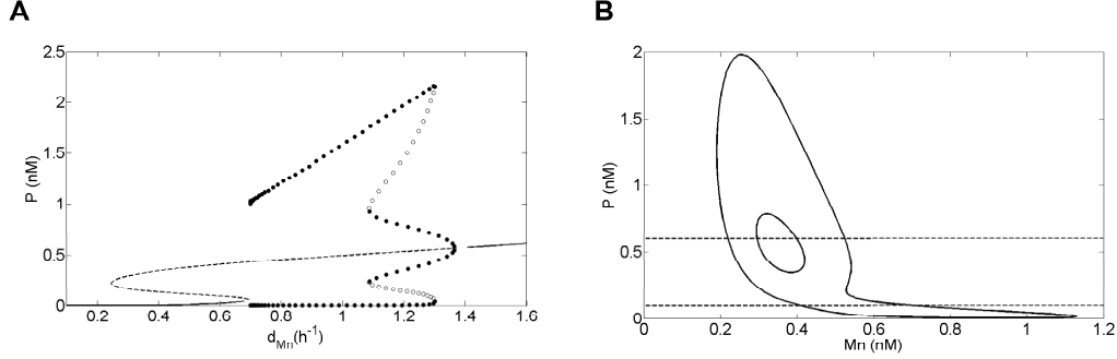
(A) Bifurcation diagrams of p53 level as a function of d_{Mn} for the OAK Model (Ouattara et al., 2010). Solid lines (resp. dashed lines) represent the stable (resp. unstable) equilibrium points. Bold (resp. white) dots are the maxima and minima of the stable (resp. unstable) limit cycles. The system shows a birhythmic domain for 1.09 \text{ h}^{-1} < d_{Mn} < 1.3 \text{ h}^{-1} . (B) Projection of the two oscillatory regimes on the plane (Mn,P) for d_{Mn}=1.2 \text{ h}^{-1} . The thresholds, K_{Mc} and K_{Mn} , related to P are indicated in dashed lines. The parameter values for the bifurcation diagram are K_{Mn}=0.1 \text{ nM} , K_{Mc}=0.6 \text{ nM} , k_p=5 \text{ nM}\cdot\text{h}^{-1} , k_{Mc}=0.1 \text{ nM}\cdot\text{h}^{-1} , k'_{Mc}=1.2 \text{ nM}\cdot\text{h}^{-1} , d_p=0.1 \text{ h}^{-1} , d'_p=2.3 \text{ nM}^{-1}\cdot\text{h}^{-1} , d_{Mc}=0.6 \text{ h}^{-1} , k_{in}=0.45 \text{ h}^{-1} , k'_{in}=0.4 \text{ h}^{-1} , k_{out}=0.045 \text{ h}^{-1} , K_p=0.2 \text{ nM} and V_r=10 .
