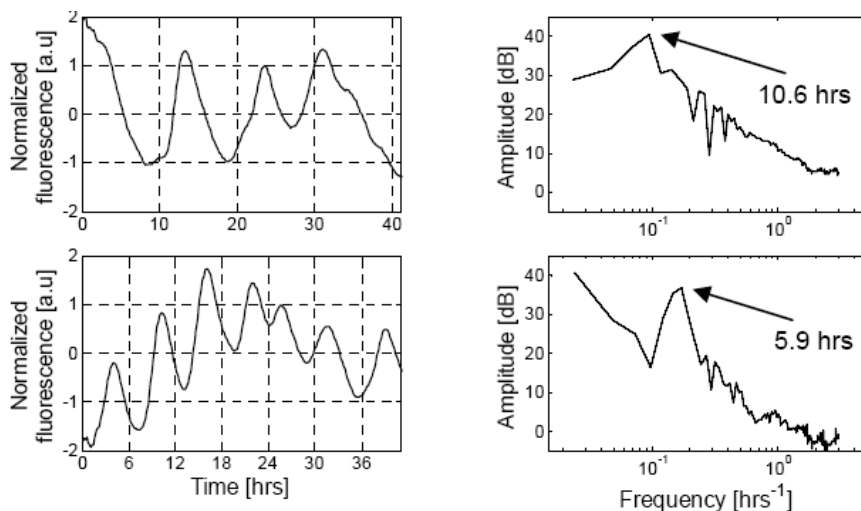
Figure 1. Experimental data from (Geva-Zatorsky et al., 2006, Fig.S3) [11]. Power spectrum of nuclear Mdm2-YFP fluorescence dynamics in individual cells. Top: an example of a cell showing fluctuations with a characteristic frequency of \sim 10 hours (exposed to 0.3Gy of gamma irradiation), and the power spectrum of the signal (by Fourier transform). Bottom: an example of a cell with multiple oscillations with a period of \sim 6 hours (exposed to 5Gy), and the power spectrum of the signal (right). Reprinted by permission from Macmillan Publishers Ltd: Molecular Systems Biology, advance online publication, 2006 (doi: 10.1038/msb4100068).
