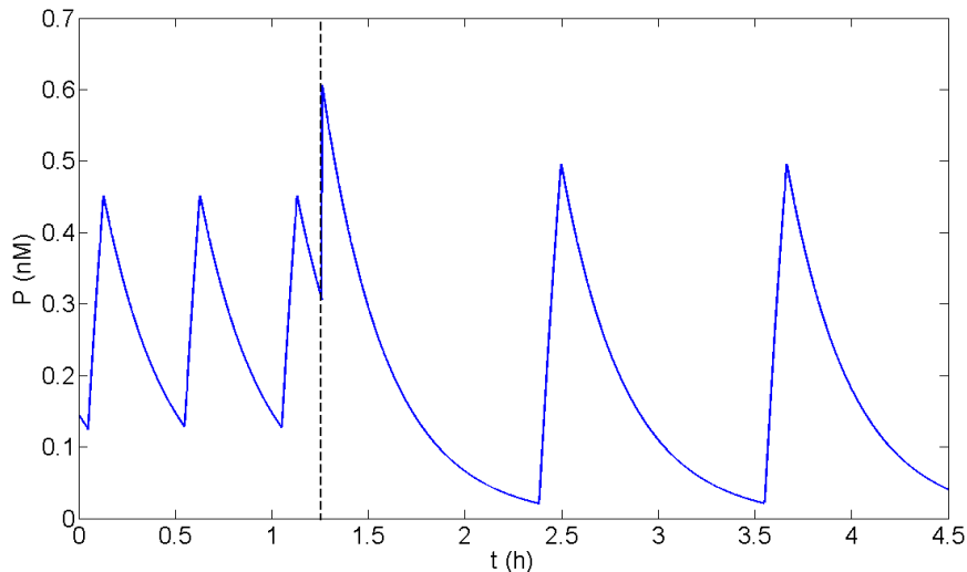
Figure 12. Permanent shift from short to long period oscillatory regime after a transient p53 pulse. Temporal simulation of p53 level for Model 3. A pulse of p53 is applied at t=1.2 h (dashed line). Before applying the pulse, the system is oscillating in the small amplitude oscillatory regime. The p53 pulse induces a shift from the small amplitude short period to the large amplitude long period limit cycle. The parameter values are indicated in Figure 9.
