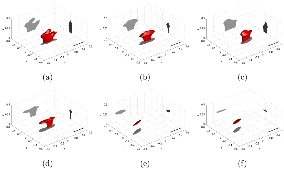
FIGURE 6.4. Experiment 2: Reconstructions of the submarine from limited aperture data ( 1/8 horizontal aperture). Blue lines in the plots indicates the wave length. (a) Conjugate incident point sources, no noise. (b) Conjugate incident point sources, 1% relative noise. (c) Conjugate incident point sources, 5% relative noise. (d) Physical incident point sources, no noise. (e) Physical incident point sources, 1% relative noise. (f) Physical incident point sources, 5% relative noise.
