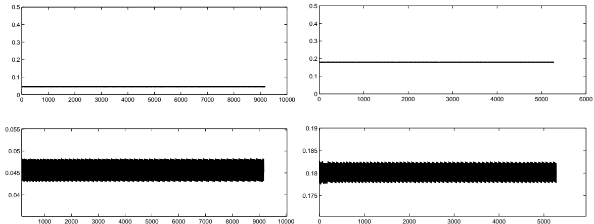
Figure 8: The velocity of the traveling plateau \sigma for different values of L with the parameters \alpha_c = 1, \alpha_S = 1, D_c = 0.1, D_S = 1 . We can see that, regardless of the numerical effect, they are almost constant. Left: L = 0.1 ; right: L = 0.4 . Top: the full scale, bottom: zoom on the oscillations.
