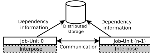
Figure 5: Transparent dependency tracking
