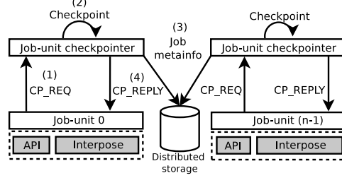
Figure 6: Independent checkpointing in XtreamGCP
