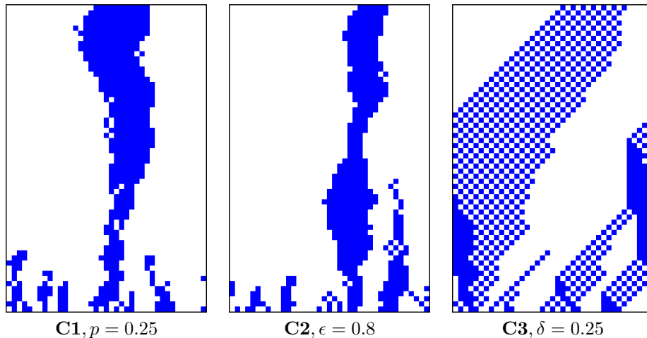
Figure 1: Space-time diagrams showing the evolution of the C1 , C2 , C3 classifiers with n = 39 , and same initial density \sim 0.4 . Time goes from bottom to top ; white cells are 0-cells and blue cells are 1-cells. (left & middle) evolution will most probably end with a good classification ( 0 ); (right) evolution will end with a good classification with probability 1 (an archipelago has been reached).
