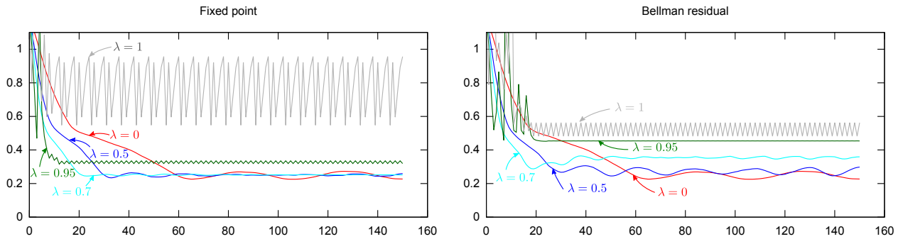
Figure 3. Chain problem. Evolution of \|\widehat{Q}_k - Q^*\|_\infty , distance between the current approximate value function and the optimal value function, for several values of \lambda , \gamma = 0.95 and with the Gaussian basis function set. Average curves of 10 runs, each run using a different set of episodes of 200 samples.
