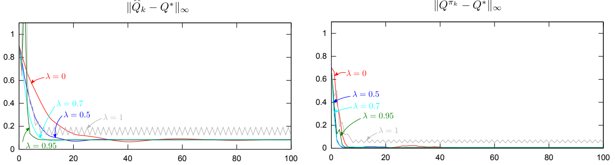
Figure 4. Chain problem. Result of FP applied with \gamma = 0.9 for several values of \lambda and the polynomial basis function set. Left: evolution of \|\hat{Q}_k - Q^*\|_\infty . Right: evolution of \|Q^{\pi_k} - Q^*\|_\infty . Average curves of 10 runs, each run using a different set of episodes of 200 samples. We observe that when the policy is the same for different values of \lambda , the value seems to converge to a limit that does not depend on \lambda . We verified this property, which does not apply to BR.
