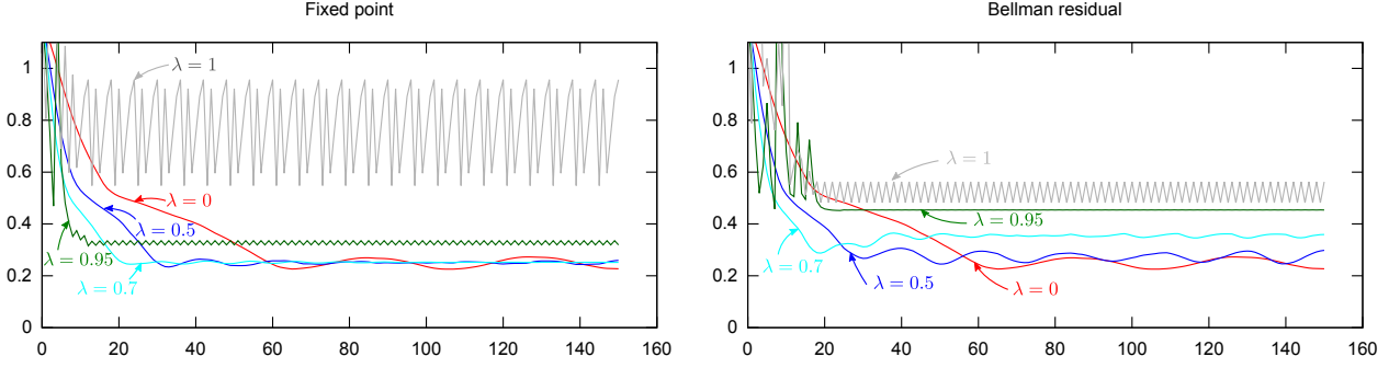
Figure 3. Chain problem. Evolution of \|\hat{Q}_k - Q^*\|_\infty , distance between the current approximate value function and the optimal value function, for several values of \lambda , \gamma = 0.95 and with the Gaussian basis function set. Average curves of 10 runs, each run using a different set of episodes of 200 samples.
