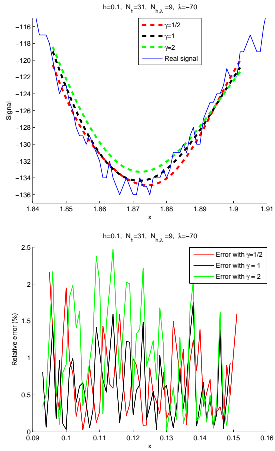
Fig. 12: Reconstruction of a part of the ABP signal (a) and relative error (b) for \lambda = -70 , h = 0.1 and \gamma = \frac{1}{2}, 1, 2
