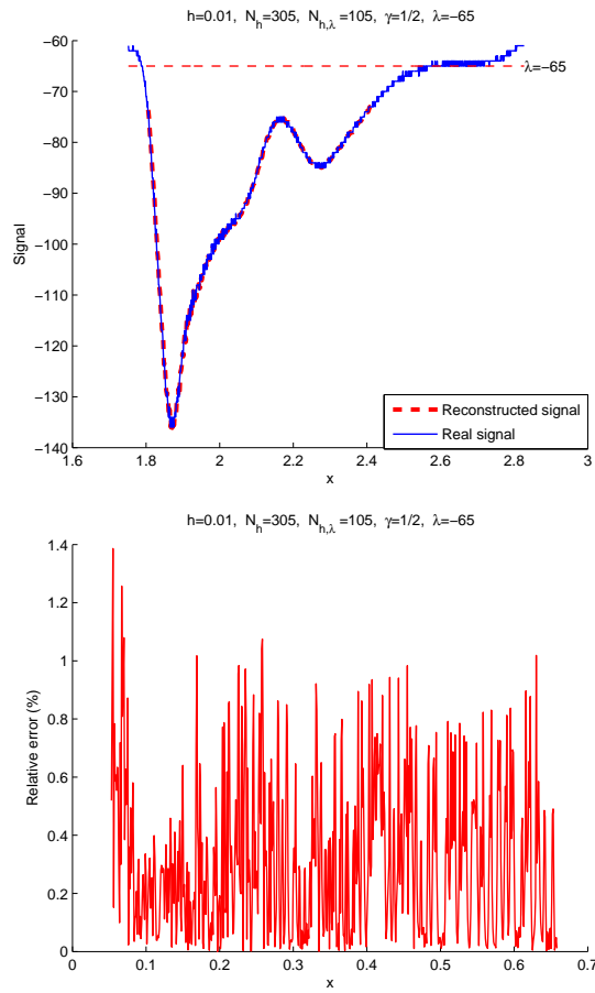
Fig. 18: Reconstruction of a part of the ABP signal (a) and relative error (b) for \lambda = -65 , h = 0.01 and \gamma = \frac{1}{2}
