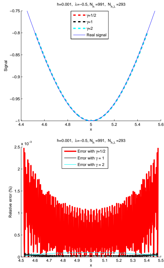
Fig. 7: Reconstruction of a part of the \text{sech}^2 signal (a) and relative error (b) for different values of \gamma and h = 0.001
