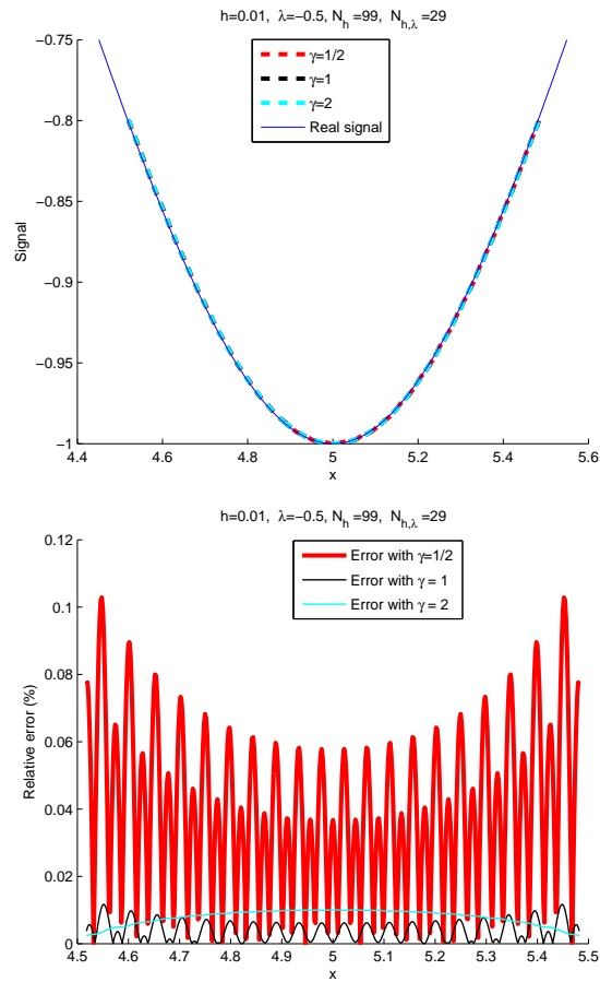
Fig. 6: Reconstruction of a part of the \text{sech}^2 signal (a) and relative error (b) for different values of \gamma and h = 0.01
