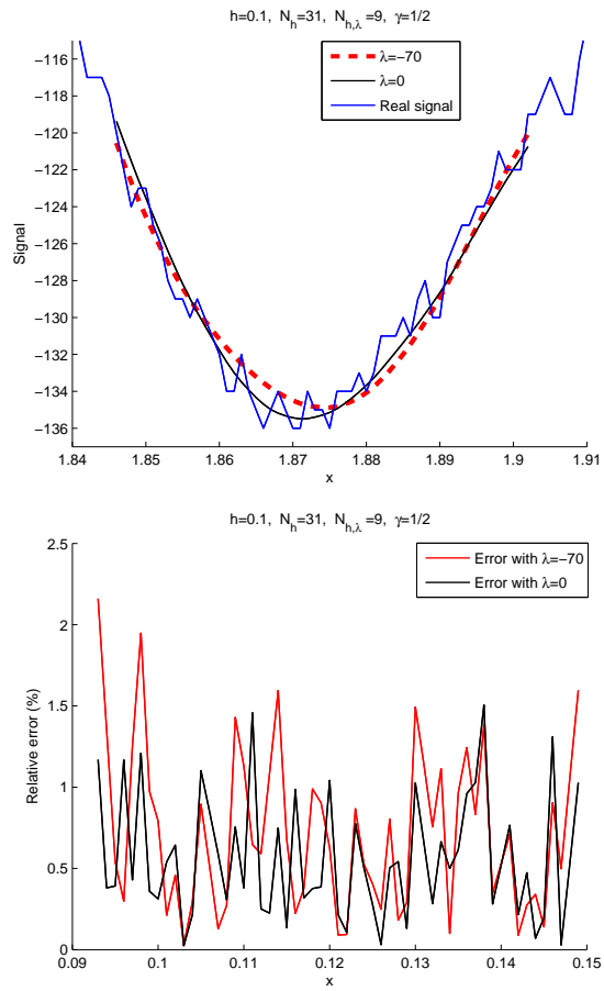
Fig. 15: Reconstruction of a part of the ABP signal (a) and relative error (b) for \lambda = 0 and -70 , h = 0.1 and \gamma = \frac{1}{2}
