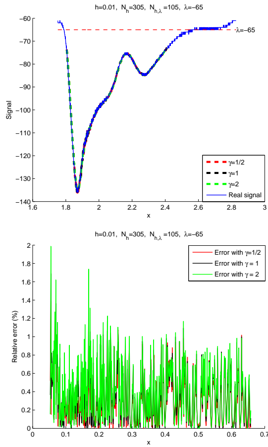
Fig. 20: Reconstruction of a part of the ABP signal (a) and relative error (b) for \lambda = -65 , h = 0.01 and \gamma = \frac{1}{2}, 1, 2
