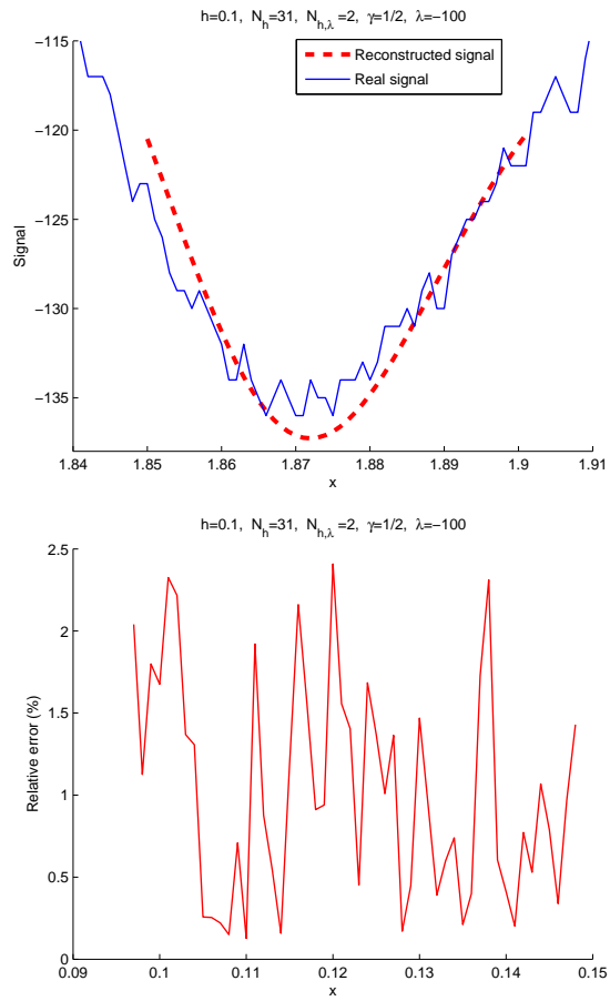
Fig. 11: Reconstruction of a part of the ABP signal (a) and relative error (b) for \lambda = -100 , h = 0.1 and \gamma = \frac{1}{2}
