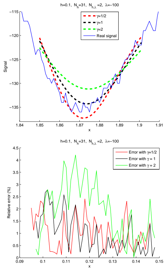
Fig. 14: Reconstruction of a part of the ABP signal (a) and relative error (b) for \lambda = -100 , h = 0.1 and \gamma = \frac{1}{2}, 1, 2
