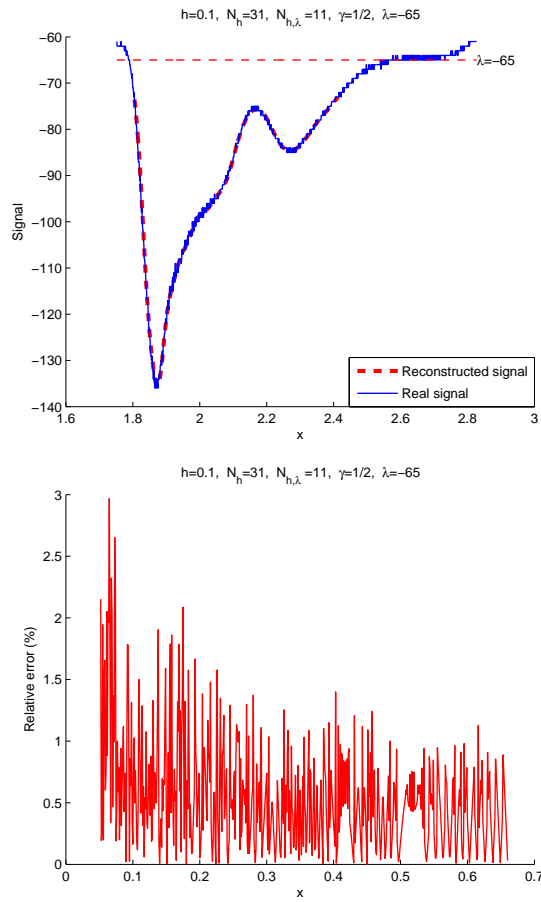
Fig. 17: Reconstruction of a part of the ABP signal (a) and relative error (b) for \lambda = -65 , h = 0.1 and \gamma = \frac{1}{2}
