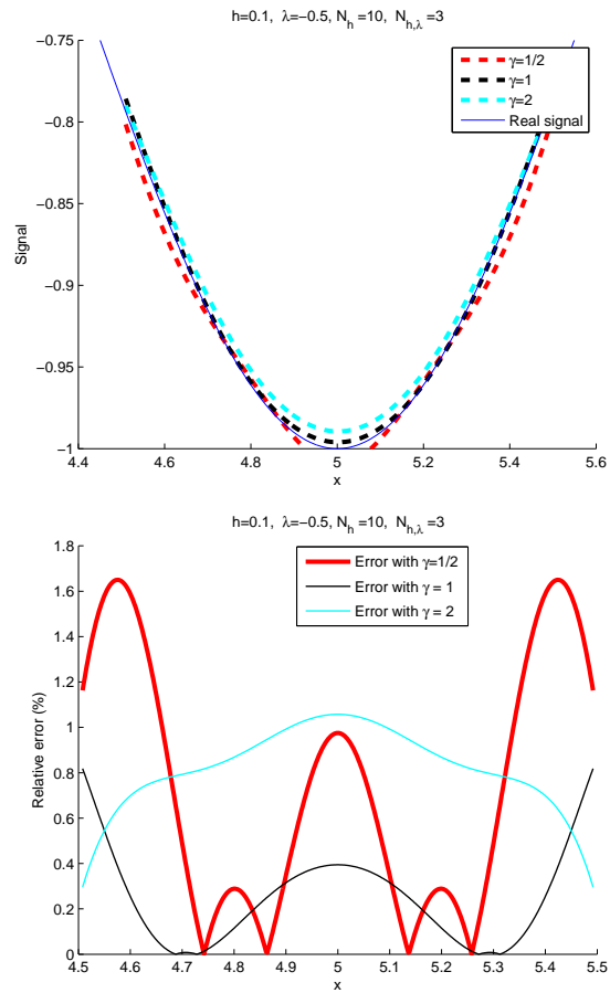
Fig. 5: Reconstruction of a part of the \text{sech}^2 signal (a) and relative error (b) for different values of \gamma and h = 0.1
