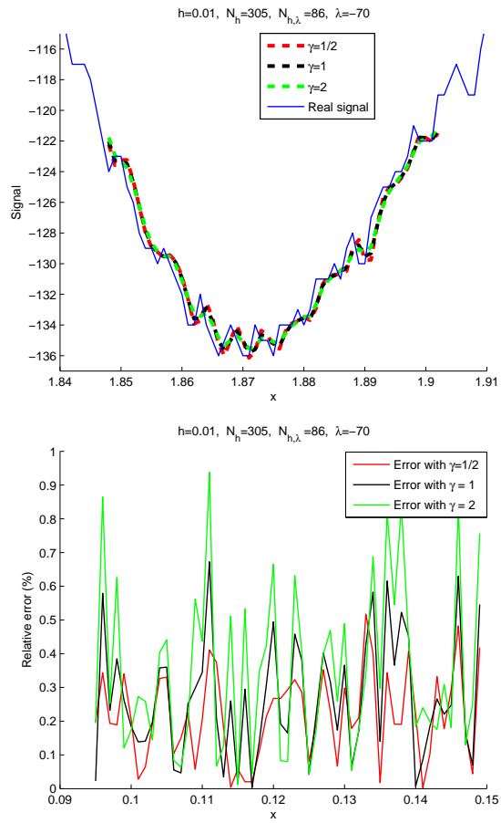
Fig. 13: Reconstruction of a part of the ABP signal (a) and relative error (b) for \lambda = -70 , h = 0.01 and \gamma = \frac{1}{2}, 1, 2
