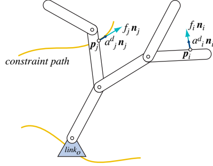
Figure 1.3: Constraints
