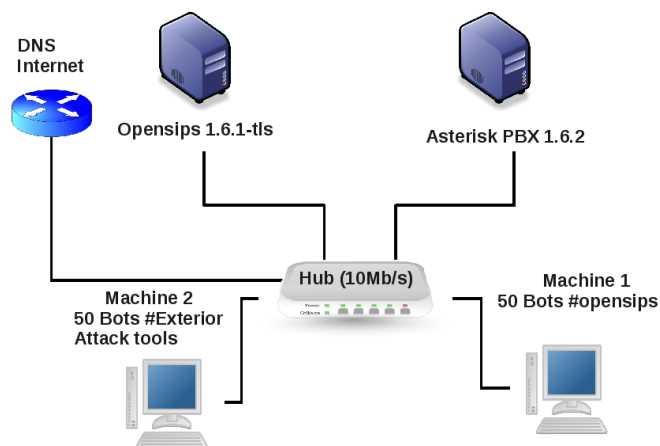
Figure 3. VoIP Test-bed
