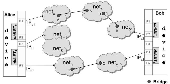
Fig. 10. Multi-network overlay through bridging
