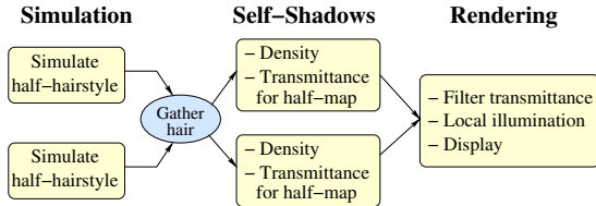
Figure 6: A parallel version of our algorithm.
