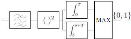
Fig. 3. PPM demodulator.
