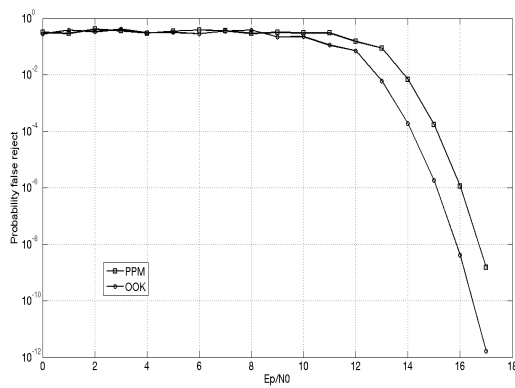
Fig. 9. Probability of false rejection of protocol A with PPM and OOK modulations, T = 2 ns, B = 1.5 GHz and N_f = 8 .
