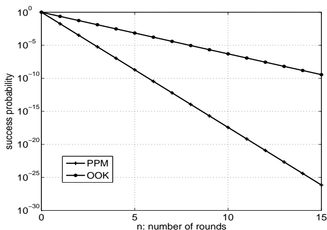
Fig. 8. Comparison of security performance of protocol A between PPM and OOK modulations, N_c = 8 , N_f = 2 and N' = 3 .
