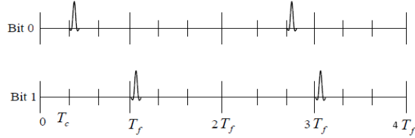
Fig. 2. Structure of a TH-UWB symbol with N_c = 3 , N_f = 4 , OOK modulation and a mapping code like Equation 1.
