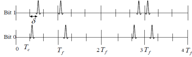
Fig. 1. Structure of a TH-UWB symbol with N_c = 3 , N_f = 4 , PPM modulation and a mapping code like Equation 1.
