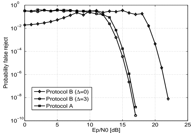
Fig. 11. Probability of false rejection of protocol B with N_f = 8 , T = 2 ns, B = 1.5 GHz and PPM modulation.
