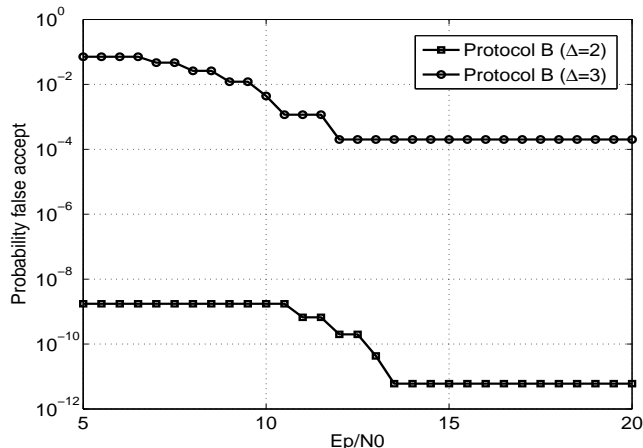
Fig. 12. Probability of false accept of protocol B over noisy channels, N_f = 8 .
