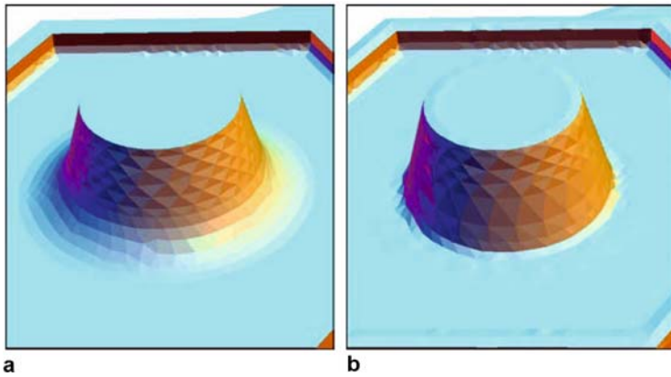
Fig. 13a,b. The rounded feature is sharpened by setting the sharpening profile curve. a Original mesh. b Sharpening result
