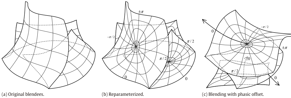
Fig. 7. Blending process.
