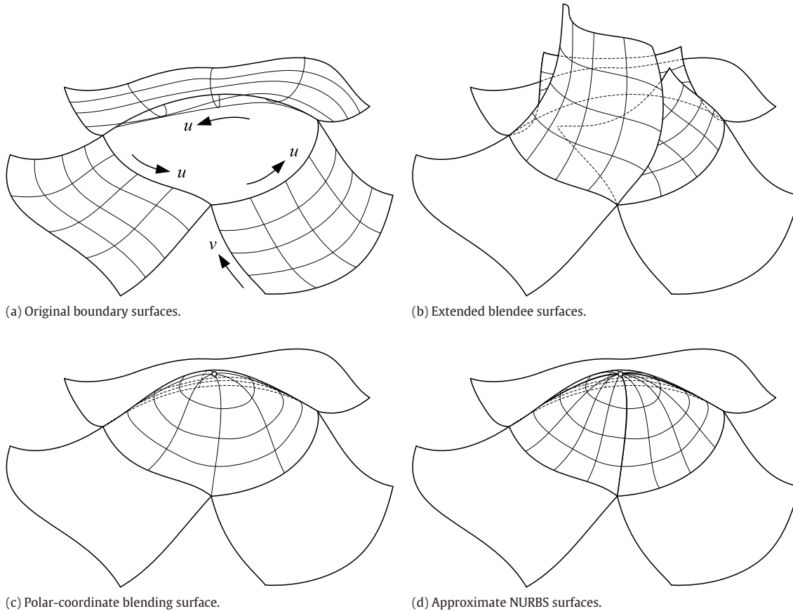
Fig. 11. Process of filling N -sided holes.
