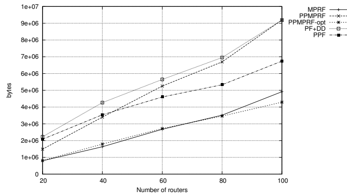
Figure 19: Broadcast: total retransmission overhead
