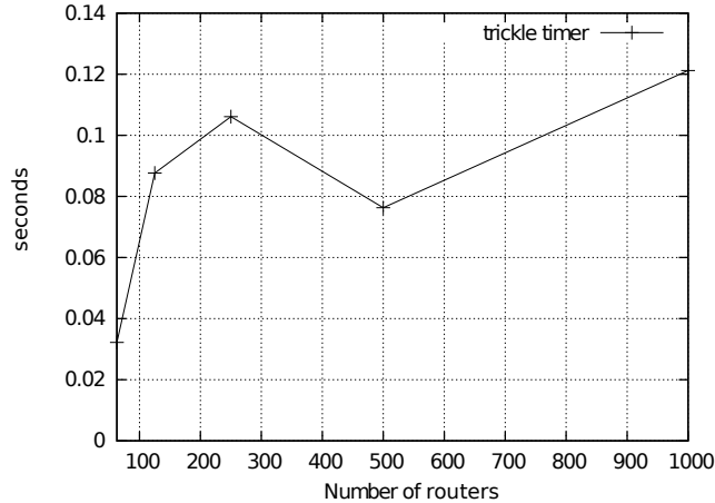
Figure 15: Unicast: delay
