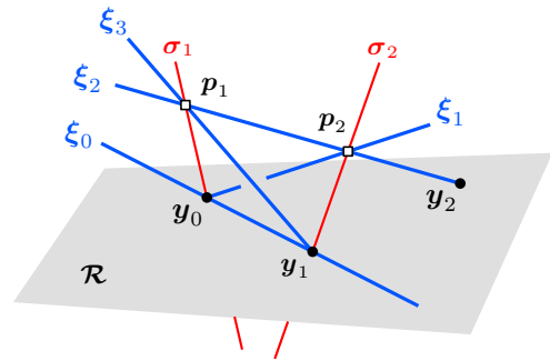
Figure 9: Two-slit camera ( p_0 = y_0 , p_3 = y_1 and y_2 = p_1 + p_2 ).
