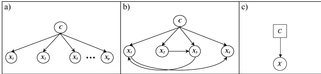
Figure 001: different bayesian network classifiers
