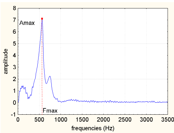
Figure 5. Amplitude ( A_{max} ) and frequency ( F_{max} ) of the maximum on the spectral curve of a tennis ball
