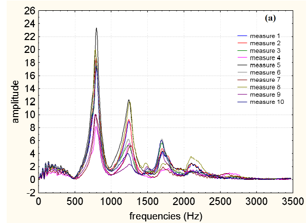
Figure 4. Variability of the spectra for repeated measurements on the same side of the same fruit
