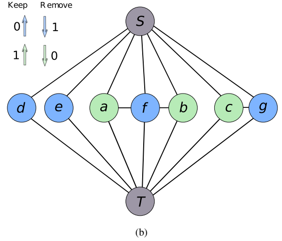
Fig. 3: (a) Image containing a current configuration \omega_{(n)} in green and a candidate configuration \omega' in blue. (b) The special graph constructed for \omega_{(n)} \cup \omega' .
