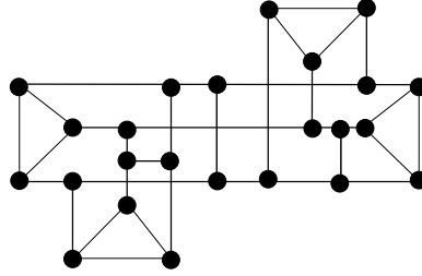
FIGURE 3. A 3-extended 3T_4
