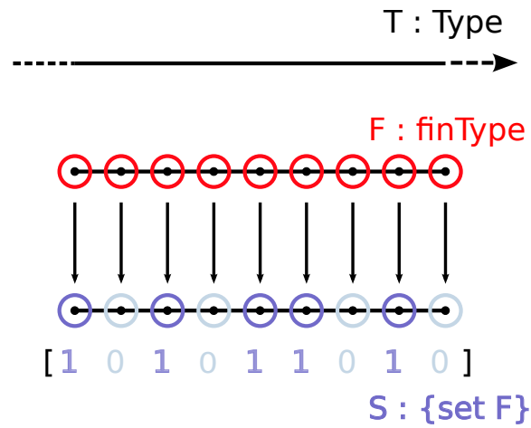
Figure 3: Finite sets as masks on finite types
