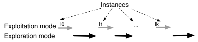
Figure 1. Continuous Search scenario
