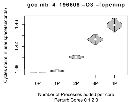
Figure 30: Observed User Execution Times for mb_4_196608 binded to the 0, 1, 2 and 3 cores
