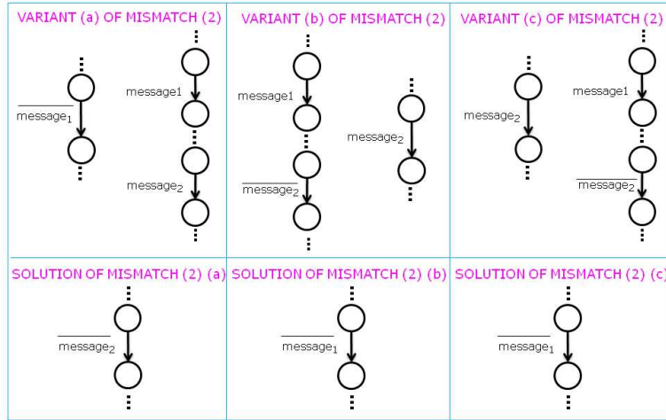
Figure 7: Variants of the Basic Mediator Pattern (2)
