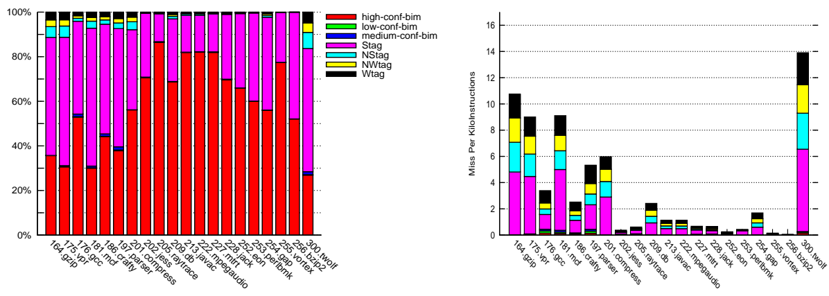
64 Kbits predictor
