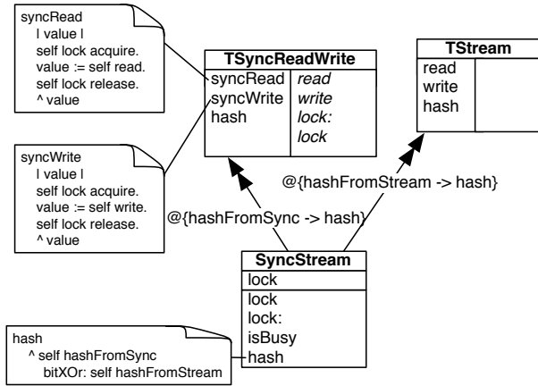
Figure 7. The class SyncStream is composed of the two traits TSynReadWrite and TStream.
