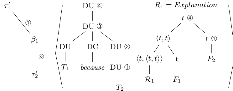
Fig. 6. Derivation tree and derived tree pair for a DNF of the form C_1 because C_2 (using the functor \mathcal{R}_1 in the semantic tree)
