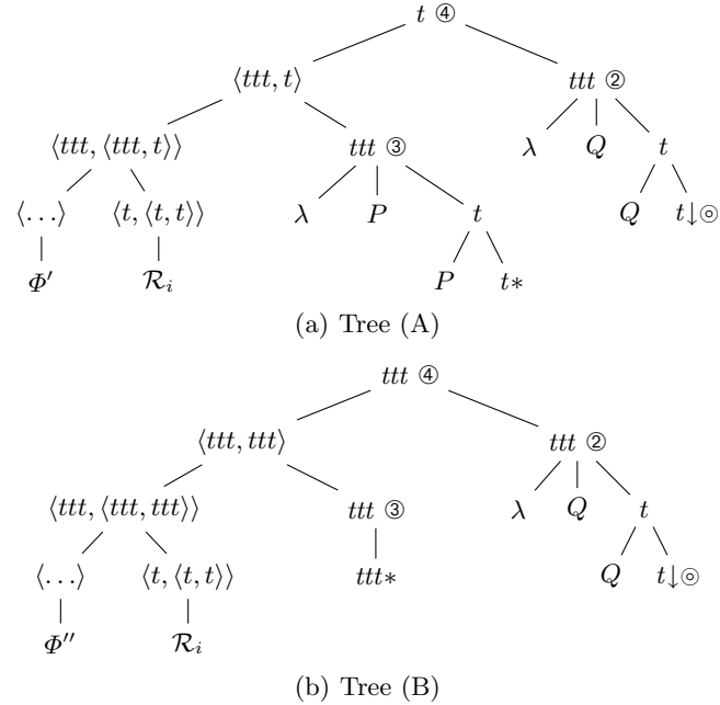
Fig. 7. Semantic trees (A) and (B) anchored by \mathcal{R}'_i = \phi'(\mathcal{R}_i) and \mathcal{R}''_i = \phi''(\mathcal{R}_i)
