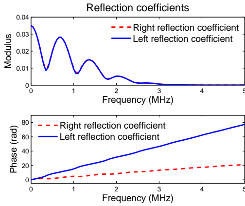
Fig. 5. Simulated engineering reflection coefficients r_{le}(k) and r_{re}(k) for R/L and G/C depicted in Fig. 4.
