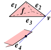
Fig. 4. The extremal case of type FvE vertex.
