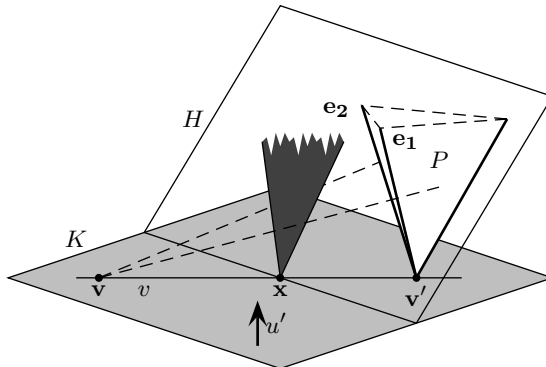
Fig. 9. The silhouette of the polytope P from \mathbf{v} projected on H is inside the cone of the projected salient edges. If the salient edges are in the half-plane u' \cdot x \geq 0 , so is the polytope.
