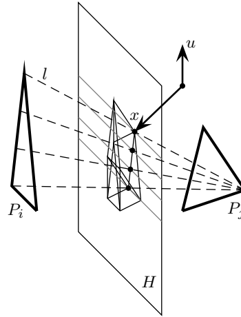
Fig. 6. The figure on plane H represents the intersections with H of the maximal free line segments corresponding to the skeleton arcs and vertices supported by P_i and P_j . The value of each of the maximal free line segments is defined by a linear function of its intersection with the plane H .
