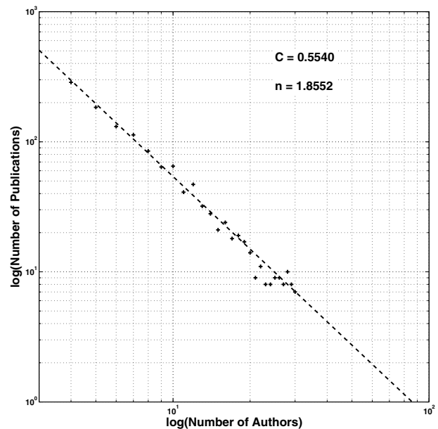
Fig. 2. Log-Log plot of the number of author and the number of publications
