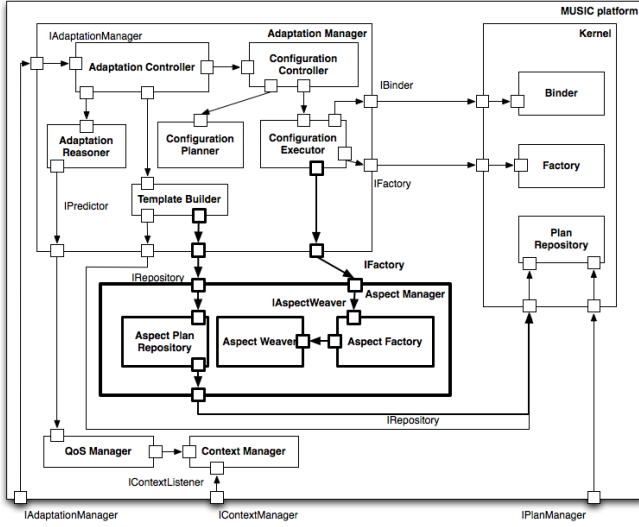
Fig. 2. Extended Middleware Architecture.
