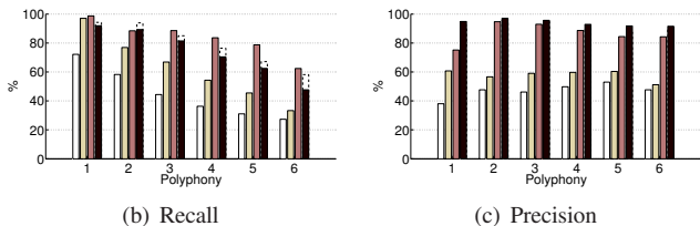
Fig. 7. Multipitch estimation results with unknown polyphony: for each algorithm, the F-measure, the precision and the recall are rendered as a function of the true polyphony. For the proposed method, the performance on the training set is plotted using a dashed line.
