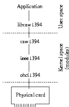
Figure 1. The 1394 hierarchy
