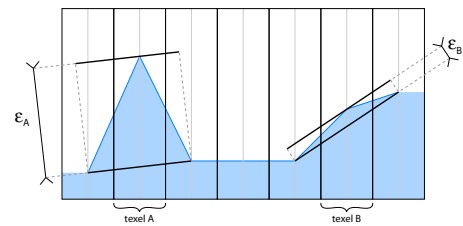
Figure 7: For texel A and B, the safety radius is 0 as we can clearly find rays intersecting the heightfield twice arbitrarily close to the texel's centers. Setting a non zero radius will create incorrect silhouettes of size \epsilon .
