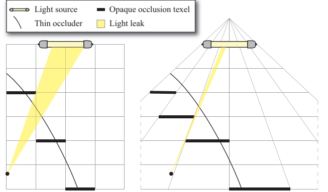
Figure 4. Orthogonal projection (left) causes more light leaks than perspective one (right).
