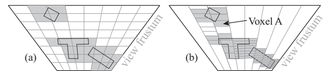
Figure 2: Uniform vs. local slicing (a) columns are sliced uniformly using the camera's depth range, yielding a "regular grid" and coarse voxels (b) each column is sliced using local depth range, yielding a "distorted grid" and generally finer voxelization.
