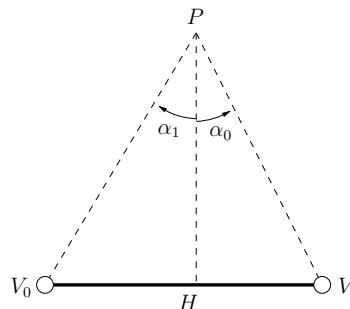
Figure 3. The field function that results from the convolution of 1/d^3 along a line-segment skeleton is based on the distance between P and its projection point H , and on the signed angles \alpha_0 and \alpha_1 .
