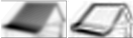
Figure 11. Intermediate maps used for the house illustration of Figure 1. Left: The omni-directional density map. Right: The gradient image computed on this map. This image is not actually stored as gradient computations are made on the fly.
