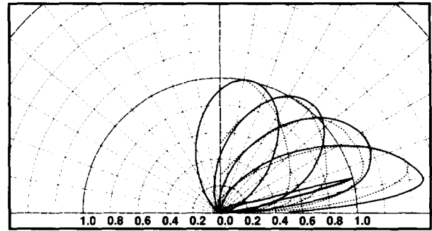
Figure 8: Normalized BRDF's of roughened aluminum as obtained from theory (solid lines) and experiment (dashed lines) for incidence angles of \theta_i = 10^\circ, 30^\circ, 45^\circ, 60^\circ, and 75^\circ . \lambda = 0.5\mu\text{m} . This is the same surface as in Figure 7. The surface shows strong directional diffuse and emerging specular reflection at this wavelength.
