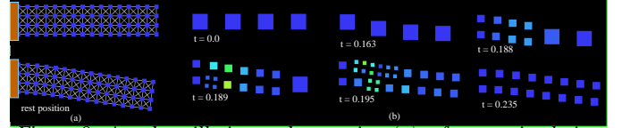
Figure 9: A rod oscillating under gravity. (a) reference simulation made with 256 particles. (b) adaptive simulation snapshots.
